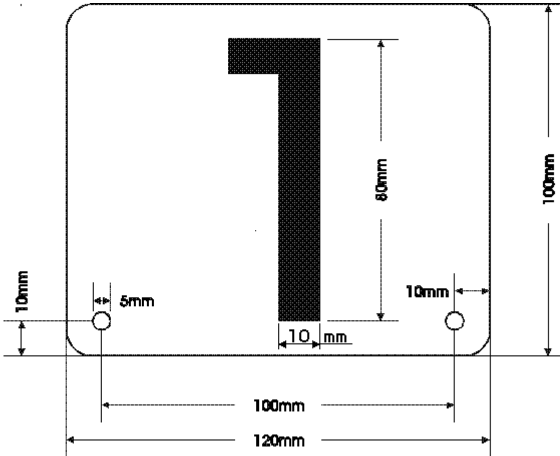
Drawing 2: Number plate for category FSR.
